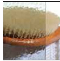
Soft Hammered/Aquatic
